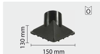
tobera triangular
